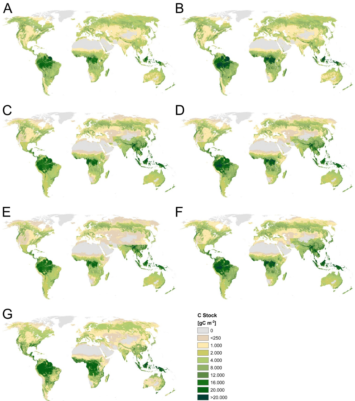
Extended Data Figure 3 | Actual biomass stock maps used in the study. a , FRA-based map. b–d , Maps based on refs 16 ( b ), 6 and 8 ( c ), and 7 and 8 ( d ). e , Remote-sensing-derived minimum. f , Remote-sensing-derived
