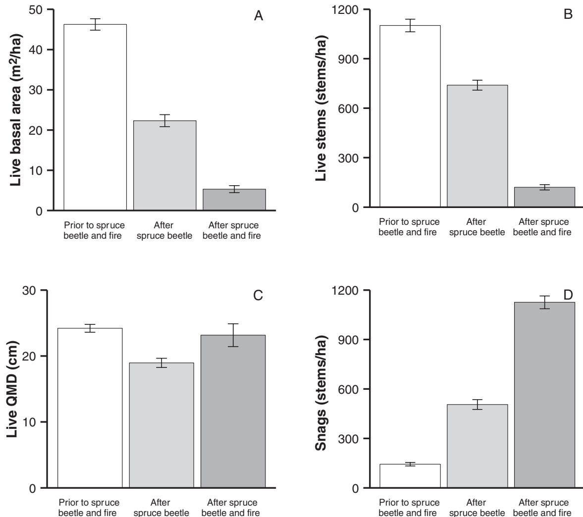
FIG. 2. Stand structure characteristics prior to spruce beetle outbreak and fire, after spruce beetle outbreak, and after spruce beetle outbreak and fire for all plots ( n = 143 ). Pre-outbreak and pre-fire characteristics were reconstructed with the criteria presented in Appendix S2. All values are mean averages and 95% confidence intervals.
