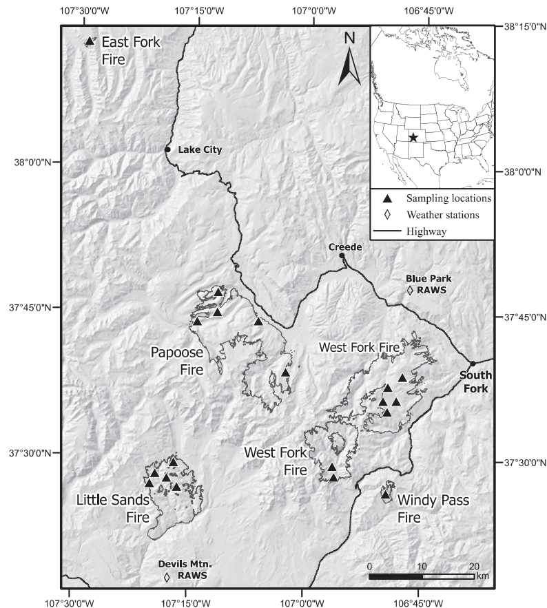
FIG. 1. Location of the five subalpine fires studied and the two weather stations (RAWS, Remote Automatic Weather Stations) used to assess burning conditions in the southern Colorado Rocky Mountains, USA. All fires burned in the summer of 2013 with the exception of the Little Sands Fire that burned in 2012. The insets display the location of the study area in North America and Colorado.
