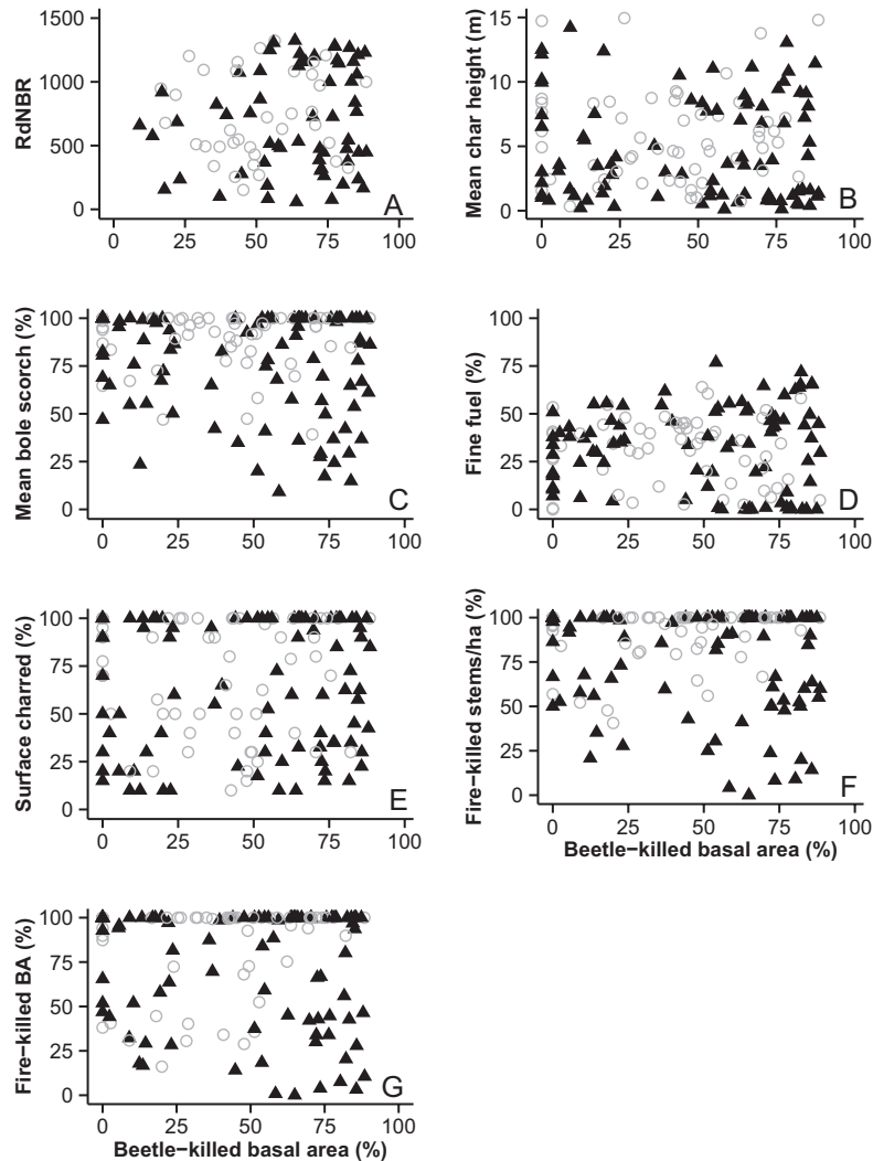
FIG. 3. (A–G) Fire severity measures plotted against spruce beetle killed basal area under moderate and extreme burning conditions (moderate, circle; extreme, triangle) in an early, gray-stage spruce beetle outbreak in subalpine, spruce-fir forests. RdNBR is relative differenced Normalized Burn Ratio. Percentage of fine fuel measures the remaining fine fuel (<1 cm) attached to the tree bole. BA is basal area.
