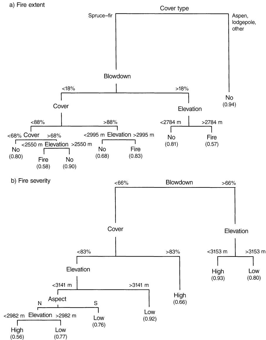
FIG. 2. Classification trees of (a) fire extent (normalized difference burn ratio [NDBR] values >1 ). The model misclassification rate was 9.3% vs. the majority misclass of 13.4%. (b) Fire severity (high NDBR values \geq 3 vs. low NDBR values <3 ). The model misclassification rate was 13.5% vs. the majority misclass of 44.7%, \kappa_{MD} = 0.63 (MD, model development; SE = 0.0449 ; z score = 14.0432), \kappa_{MV} = 0.39 (MV, model validation, SE = 0.0449 ; z score = 8.58044). The length of horizontal lines is proportional to the explained variance. Each terminal node is labeled according to the predominant classification of (a) fire occurrence (fire or no fire) or (b) severity (low or high). Parenthetical numbers indicate the probability of that classification. The figure depicts trees trimmed to 10 terminal nodes. Complete trees were pruned based on the cost-complexity measure and included 133 terminal nodes for fire extent and 55 terminal nodes for fire severity.
