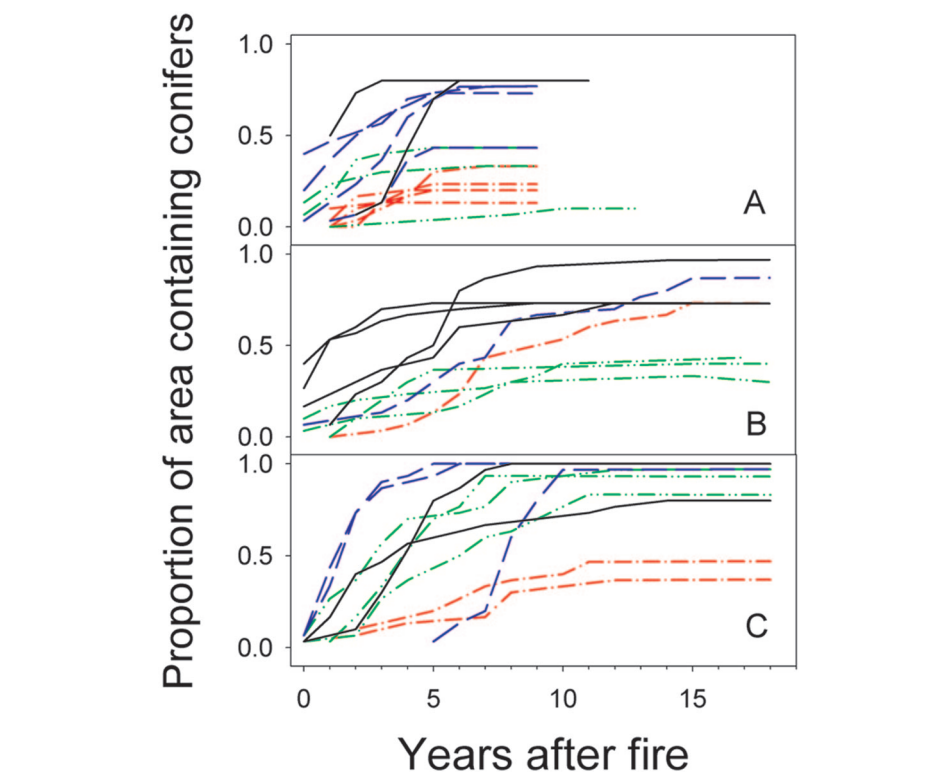
Figure 4. Changes in conifer stocking over time since wildfire (stocking = proportion of 1/600 ha cells in each plot containing one or more established conifers). The lack of similarity among shape of curves or peaks in years after fire suggests the importance of local controls, i.e., plot level variation. (A) Establishment after fires of 1992–1996 on low-elevation sites; (B) establishment after fires of 1987 on low-elevation sites (Douglas-fir and Douglas-fir/tanoak series); (C) establishment after fires of 1987 on high-elevation sites (white fir series) in the Klamath-Siskiyou region. Red (single dotted), green (double dotted), blue (long dash), and black (solid) lines indicate quartiles of increasing total seedling density (as opposed to stocking) observed at the time of our survey. Because of variation in spatial distribution of seedlings within a plot, a high seedling density did not always result in a high proportion of area occupied.
