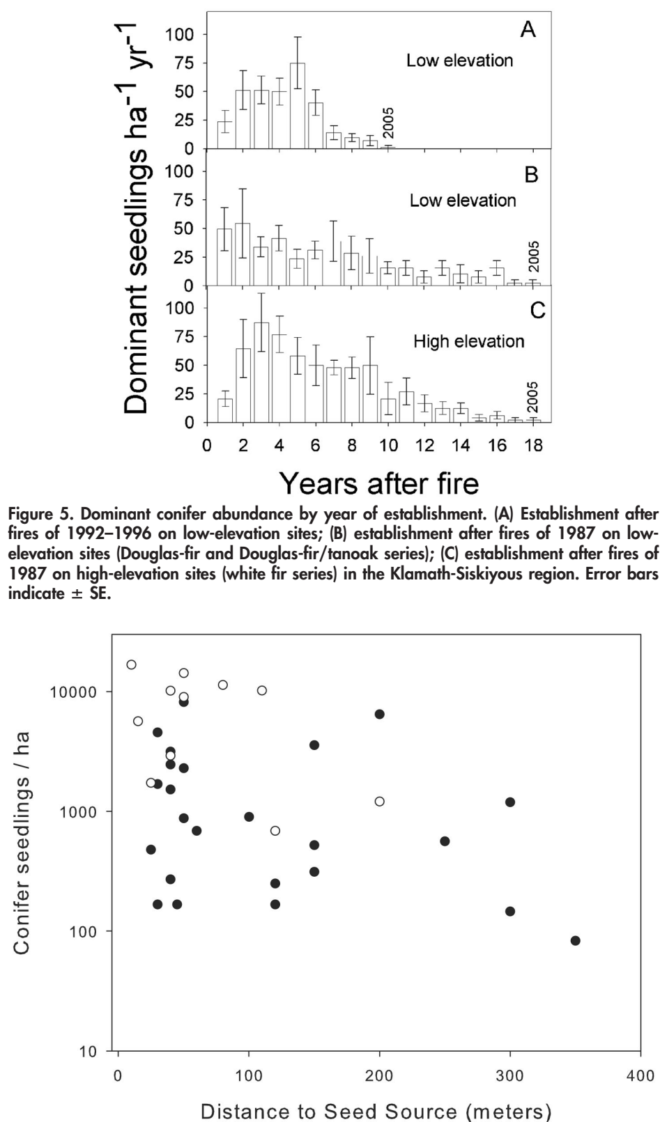
Figure 6. Tree density (tph) in relation to distance to seed source (m) for two plant associations, Douglas-fir and Douglas-fir/tanoak series (closed circles) and white fir series (open circles).
