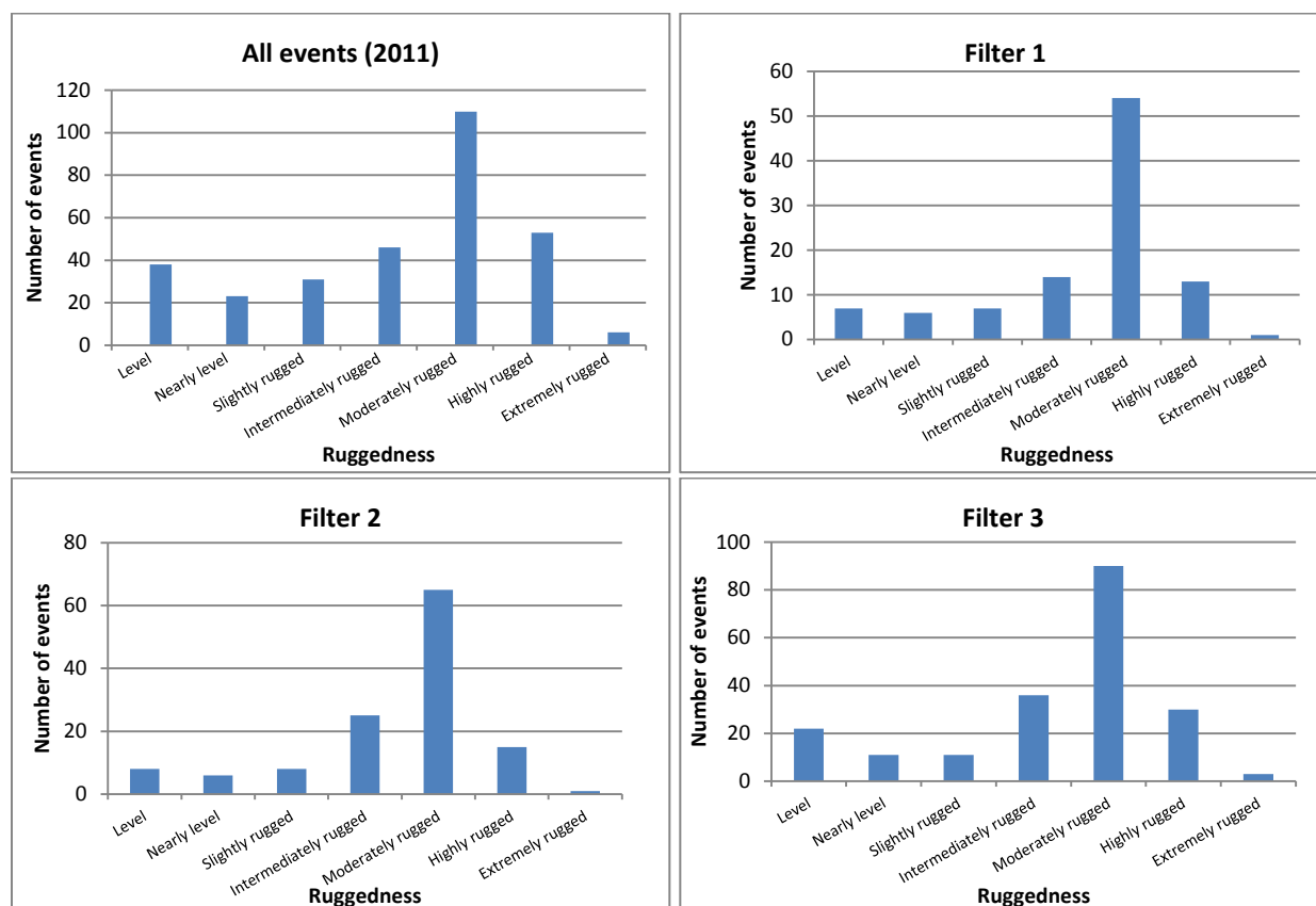
Figure 2.2. Comparison of subsets of jaguar events against jaguar habitat variable: terrain ruggedness
