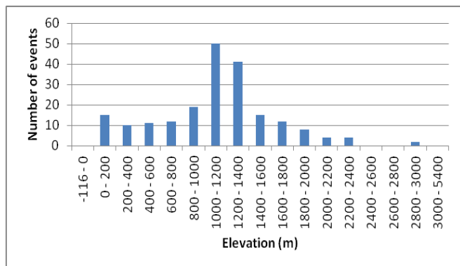
Figure 2.4. Comparison of the Filter 3 subset of jaguar events against elevation
