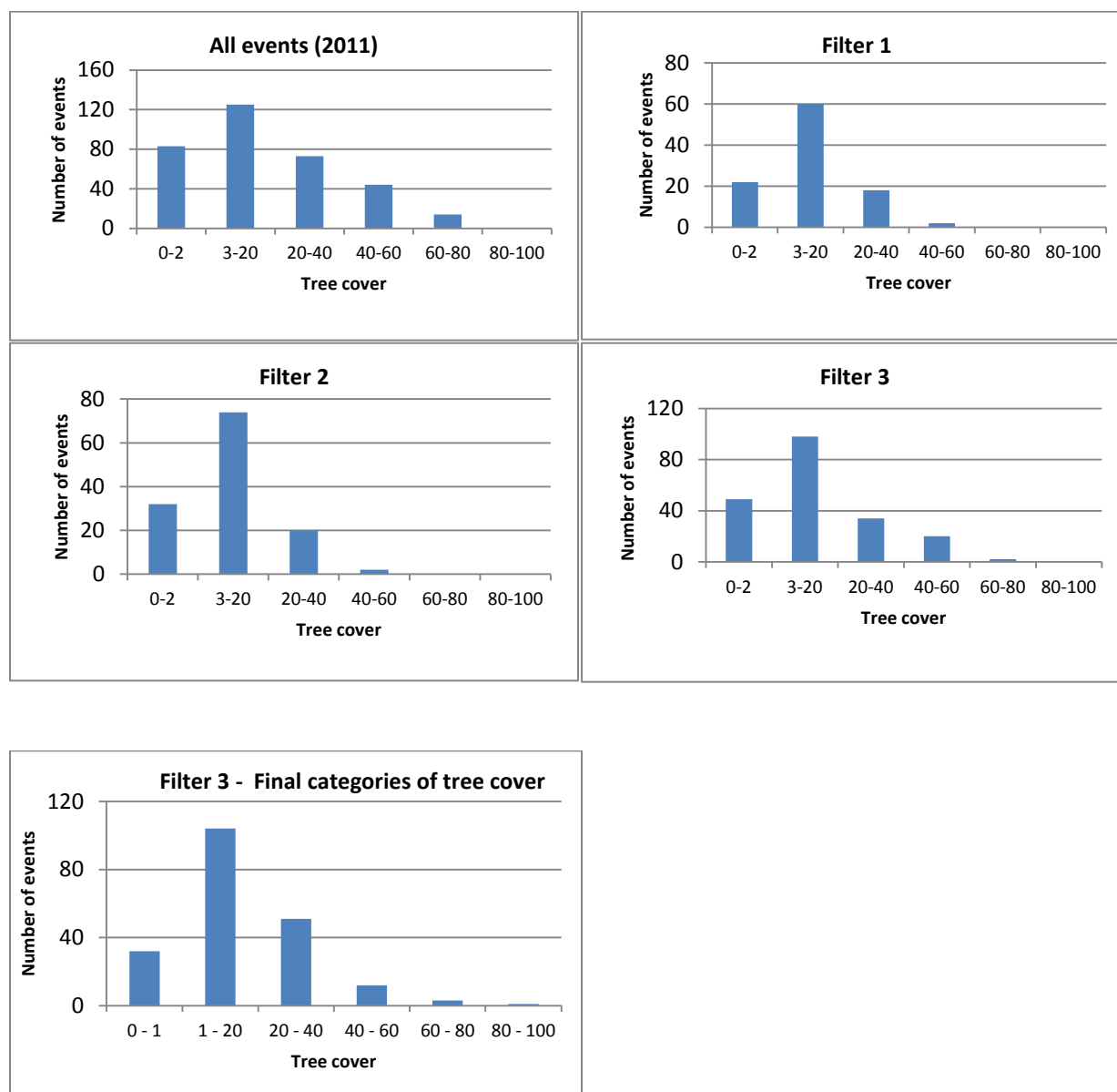
Figure 2.1. Comparison of subsets of jaguar events against jaguar habitat variable: tree cover
