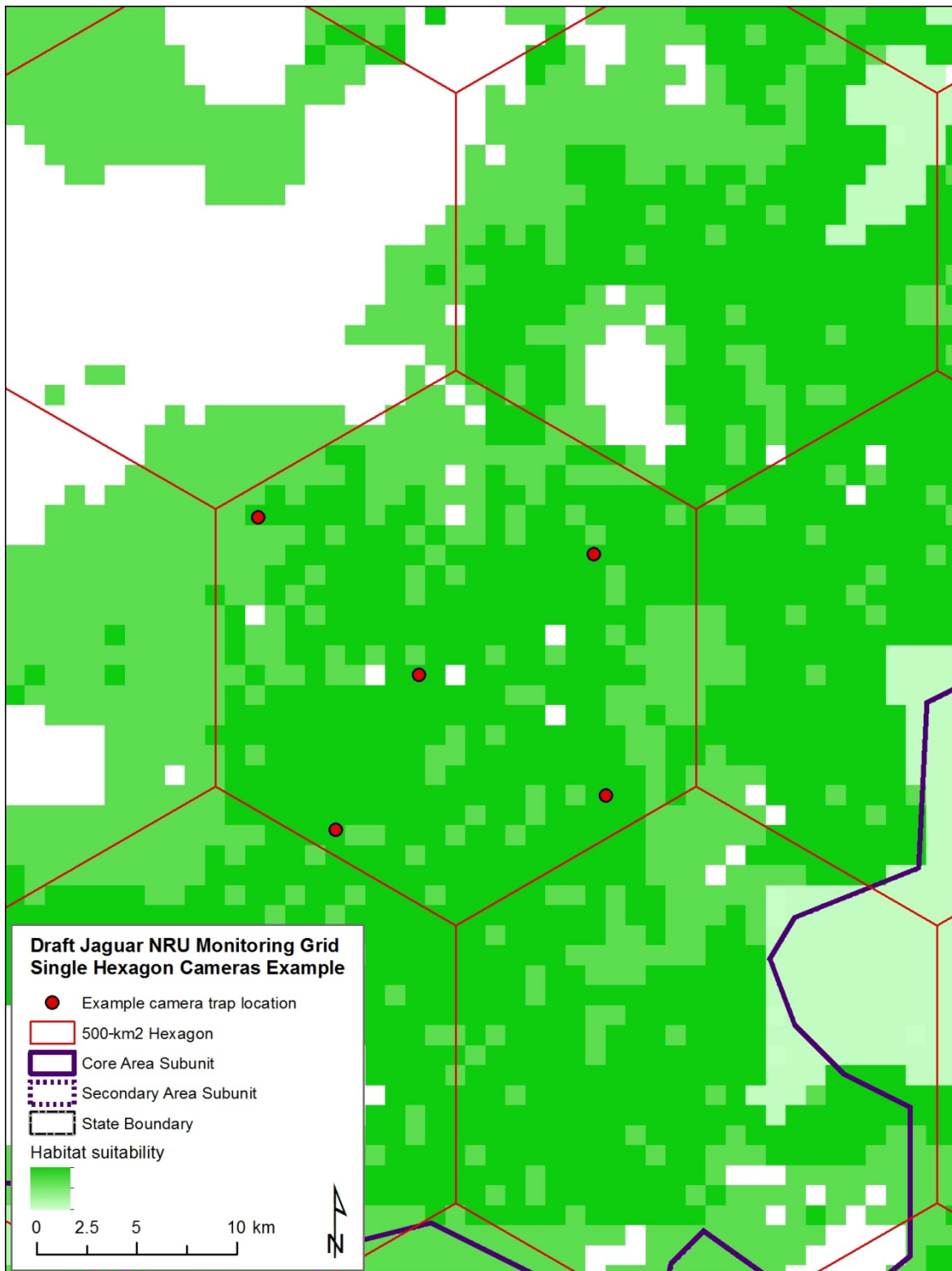
Figure 15. Individual camera-trap locations within a 500-km 2 hexagon in the 77,710 km 2 Sonora Core Area in northern Mexico. Habitat suitability index at 1-km 2 resolution, darker shades of green indicating higher suitability (Sanderson and Fisher 2013).
