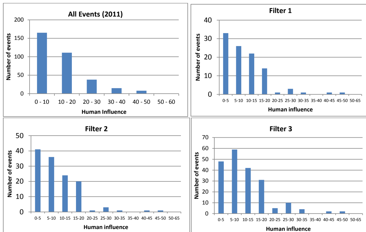
Figure 2.3. Comparison of subsets of jaguar events against jaguar habitat variable: human influence.
