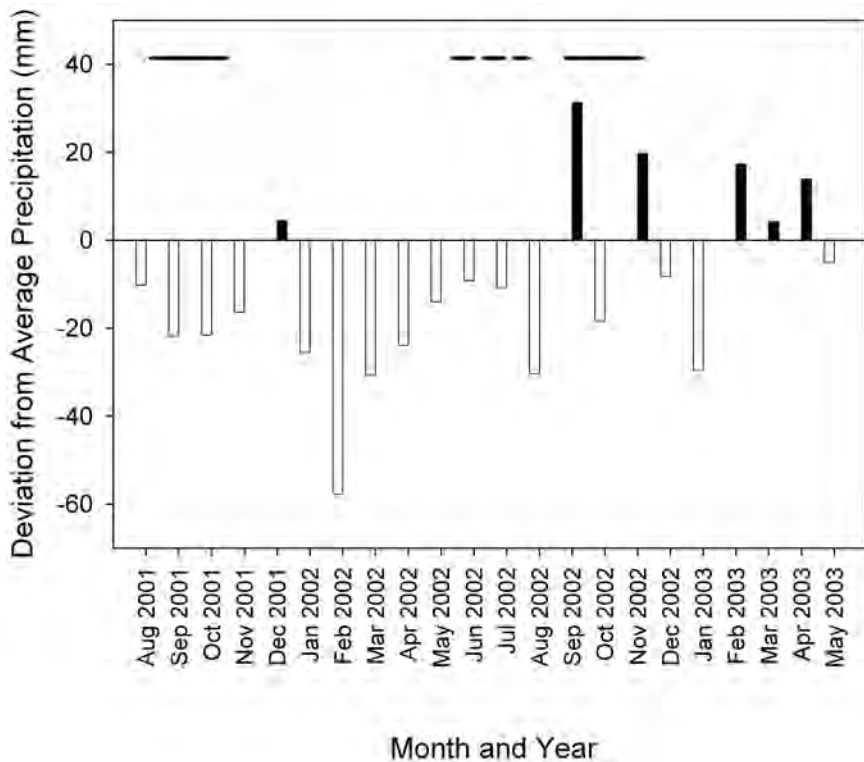
Figure 4. Deviation in monthly precipitation for August 2001–May 2003 compared to the 12-year average on Mt. Trumbull AZ, as recorded at the Nixon Flats RAWs site from 1992–2003. Black bars show above-average precipitation, white bars indicate below-average precipitation; horizontal lines at top of graph indicate timing of phenology of cheatgrass on Mt. Trumbull as observed by authors: solid line = primary germination period, dashed line = senescence and seed maturation.
