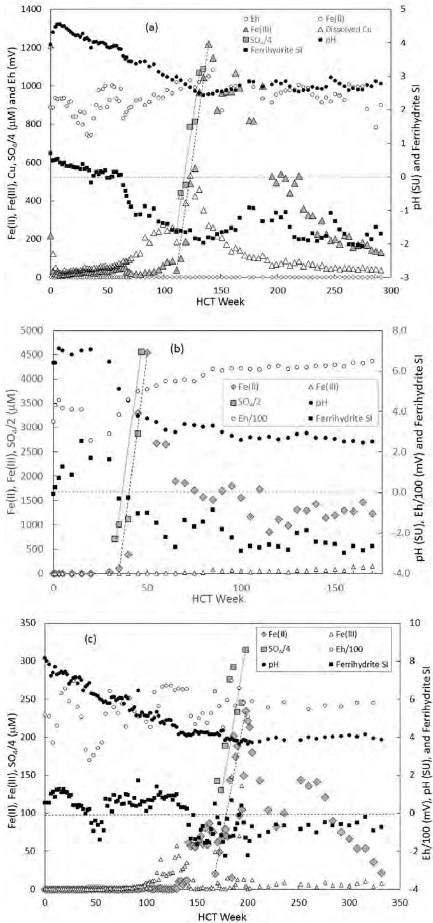
Fig. 2. Dissolved Fe species, ferrihydrate saturation index (SI), \text{SO}_4 (only during rapid increase), and Eh for (a) Pebble sample 3069-0927-0947, with dissolved Cu, (b) Buckhorn Mine sample HC-1, and (c) PolyMet Project sample 26027(616-626). Horizontal dashed line is SI = 0, and the slanted vertical dashed lines represent the part of the curve used to calculate Fe sulfide dissolution rates.
