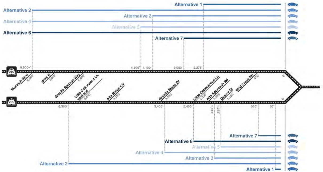
Figure 3. Queuing Results
