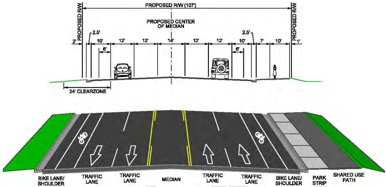
Figure 2-4. Five-lane Alternative
