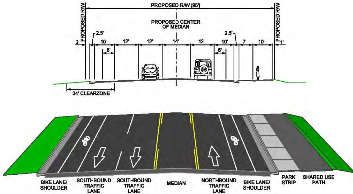
Figure 2-2. Imbalanced-lane Alternative
