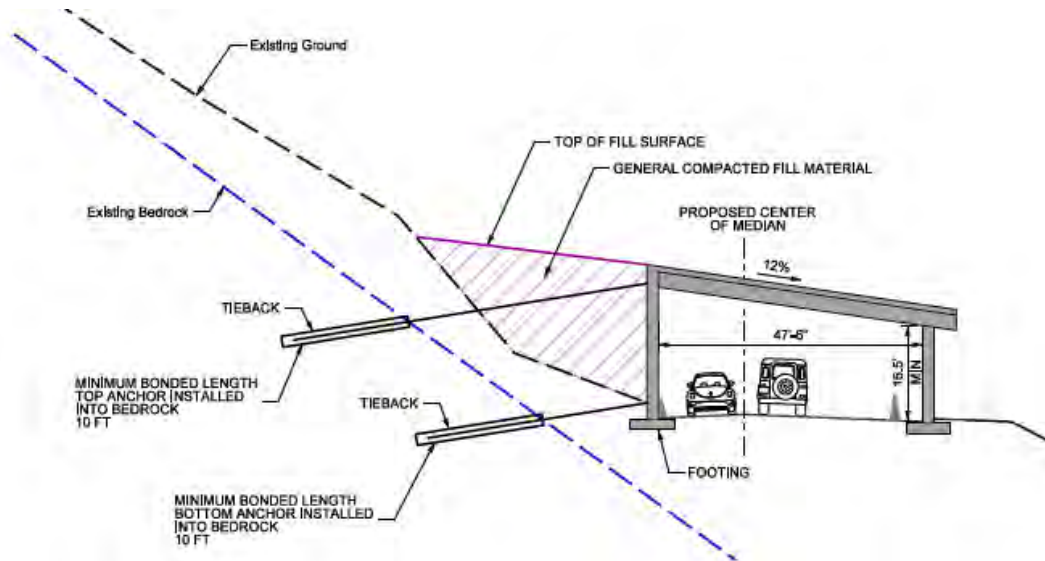
Figure 3-3. Option 1: Anchors in Bedrock
