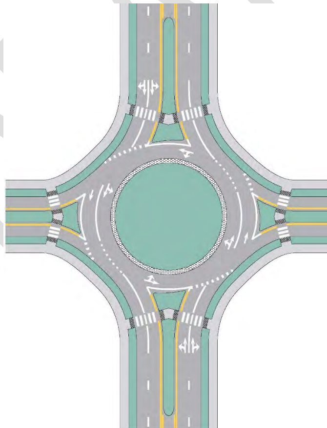
Figure 2-5. Multiple Roundabouts Alternative
