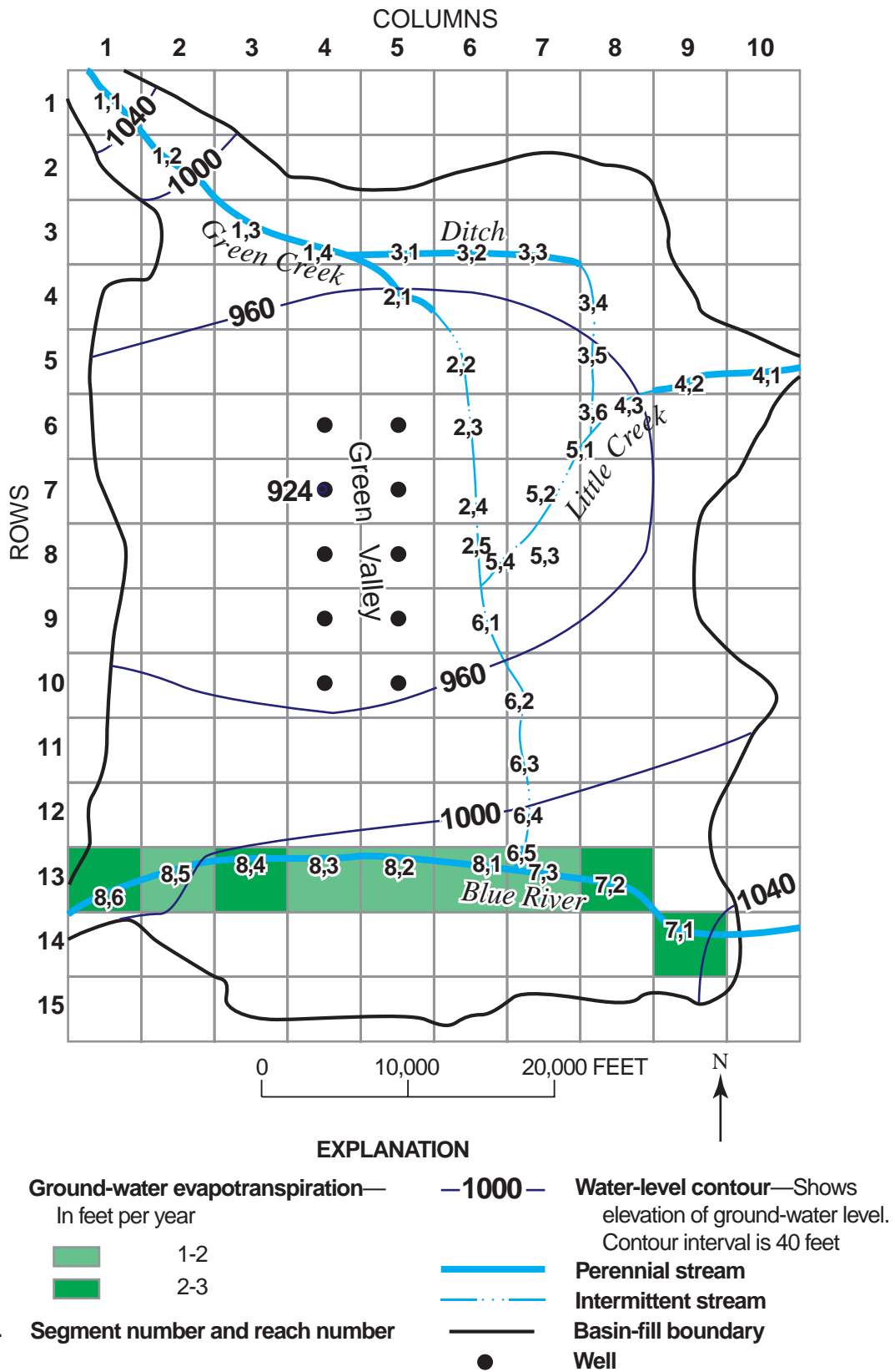
Figure 10. Model grid showing simulated water-table contours, distribution of ground-water evapotranspiration, and locations of perennial-flow reaches after 50 years of pumping (end of first stress period) for test simulation 1.
