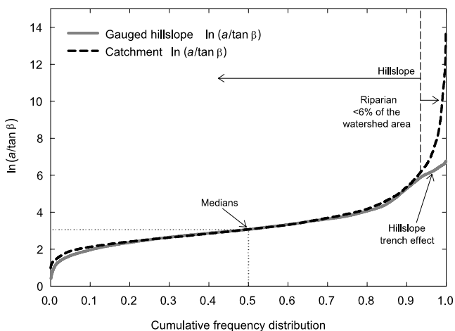
Figure 2. The gauged hillslope and hillslopes comprising a Maimai headwater catchment show comparable distributions of the topographic index \ln a/\tan\beta (mean 3.5 versus 3.2, 5% trimmed mean 3.3 versus 3.2 median 3.1 versus 3.0). The vertical dashed line denotes <6% of the catchment area; the >94% of the catchment cumulative frequency distribution toward the origin represents hillslopes and the <6% to the right represents riparian areas and strongly convergent hollows not found on the gauged hillslope.
