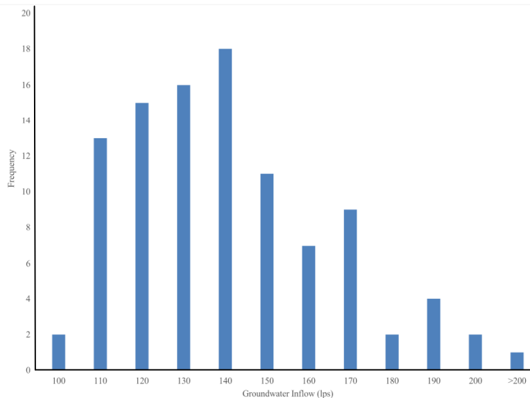
Fig. 2 Frequency histogram of NSMC pit inflow results
