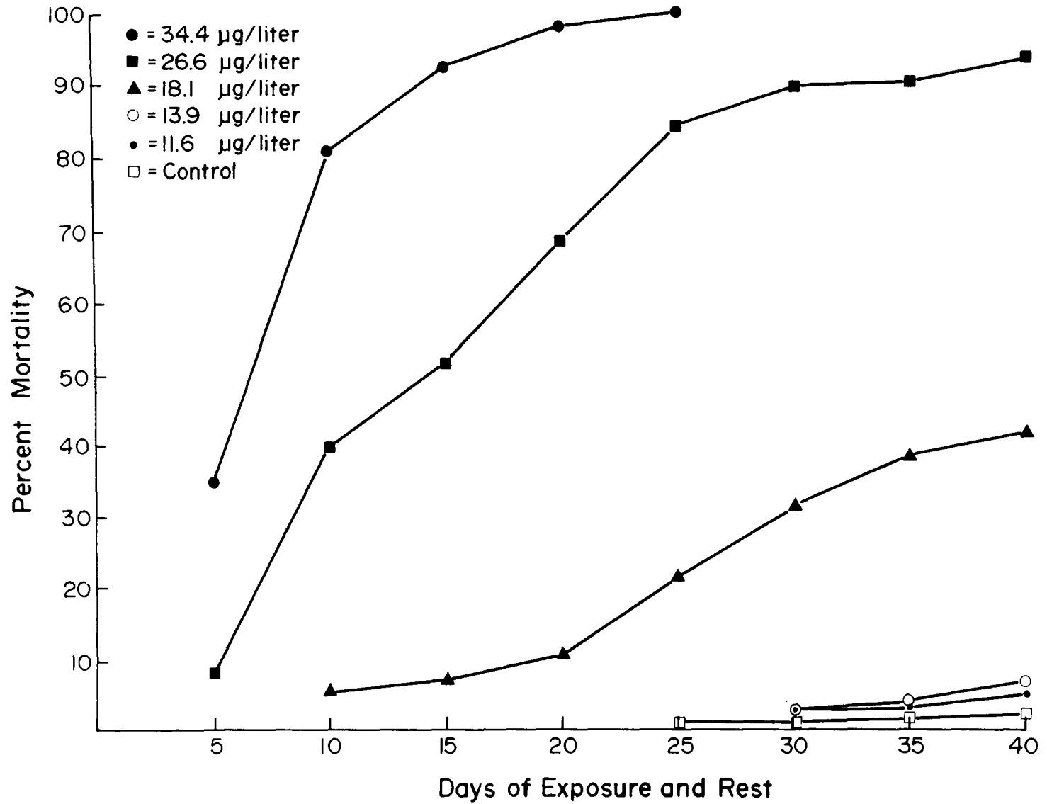
Figure 2. Mean mortality of coho salmon fry exposed to copper during the oral vaccination bioassay.
