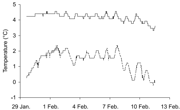
Fig. 5. Thermal profiles for two winter weeks from a gaining (solid line) and a losing (broken line) reach of Lion Creek clearly show the moderating effects (both seasonal and diel) of groundwater. The supercooled temperature of the losing reach at the end of the profile corresponded to anchor ice formation. Twenty-three bull trout redds were counted in the gaining reach, while none were found in the losing reach.
