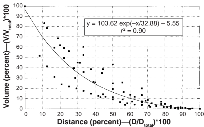
Figure 6—Dimensionless plot of volume of sediment deposition as a function of travel distance.
