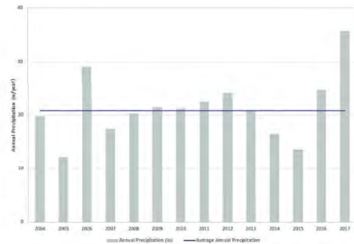
Figure 4-9: Annual Precipitation Data from the PRISM Data Set for Data Used to Simulate Average Climatic Conditions
