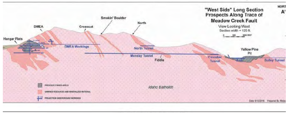
Figure 1. Mine area relative to historic tunnels. (Upper image) Historically mined areas; purple lines are underground workings. Source: DEIS Fig. 3.7-2 (Lower image) Cross-section showing tunnels. Source: Midas 2016 Plan of Restoration and Operations (PRO), Appendix D.
