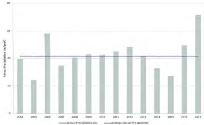
Figure 4-9: Annual Precipitation Data from the PRISM Data Set for Data Used to Simulate Average Climatic Conditions
