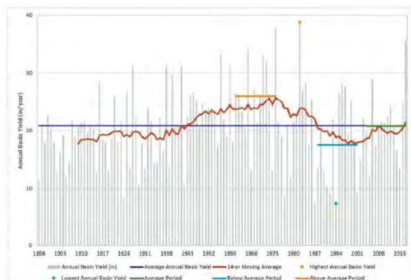
Figure 4-8: Annual Precipitation Data from the Meteoric Water Balance (BC, 2018a; 2018c)
