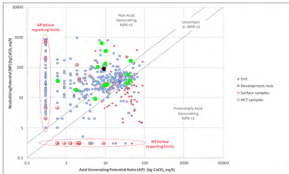
Figure 7. Waste rock and ore acid and neutralization potential. Green dots show waste rock material chosen for HCTs; the black dot is an ore sample chosen. No surface samples were chosen. Source: SRK 2017 baseline Fig. 3-8
