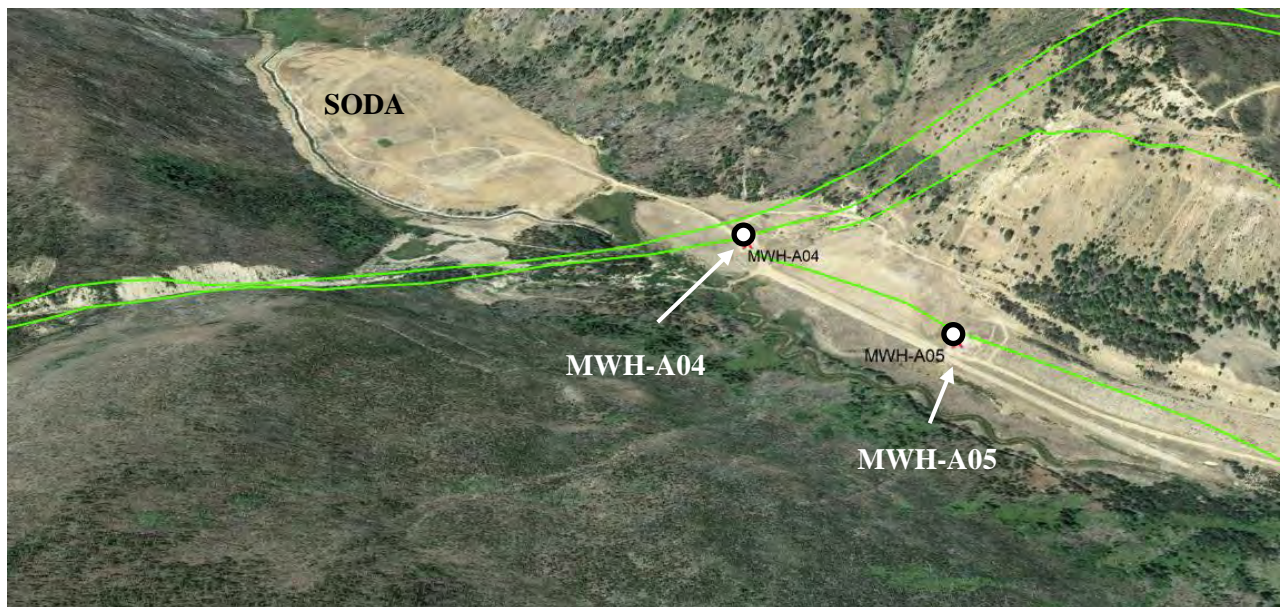
Figure 4. Location of alluvial wells with elevated dissolved Hg at old heap leaches Looking up Meadow Creek Valley; MWH-A01 is located above SODA (outside of image]. Green lines represent fault lines. Both wells are in the location of the future HF pit. Geo-location of well and fault lines relative to land features contributed by B. Prucha.
