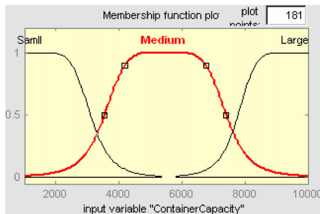
Fig. 6. Container capacity membership function.
