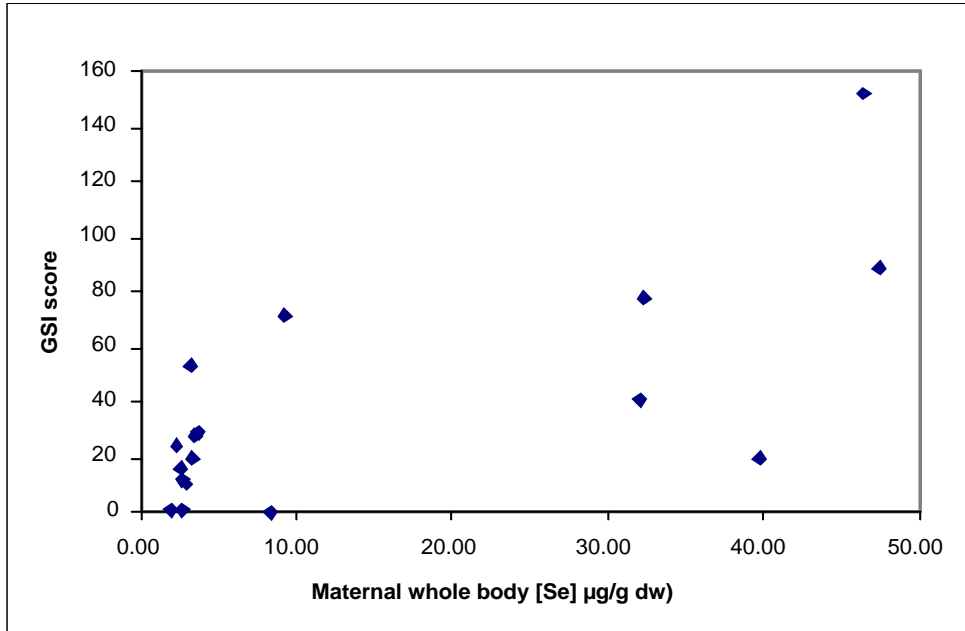
Figure E-4. Percent 2-day post-hatch larvae Graduated Severity Index (GSI) relative to maternal whole body selenium concentration
