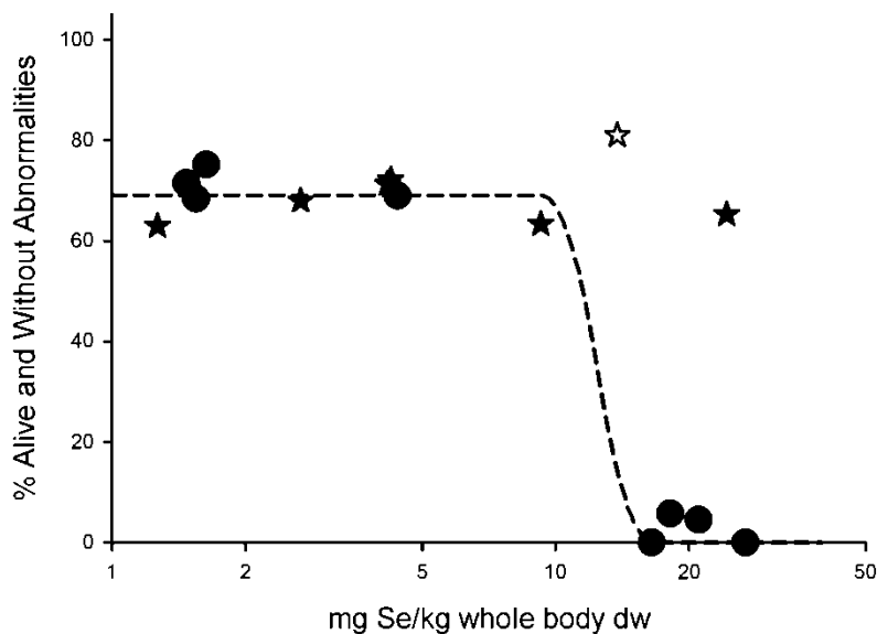
Figure 3. TRAP interpolation curve for the Table 5 whole body data. Circles denote active aqueous exposures and stars denote recovery periods. The interpolation is based on the threshold sigmoidal model, with the first interpolation point set to the HNOEC of 9.3 mg/kg whole body and the average background survival/normal of 69.1% and the second point set to the LOEC of 16.5 mg/kg and a survival/normal of 0%. The resulting EC 10 is 10.6 mg Se/kg whole body dw.
