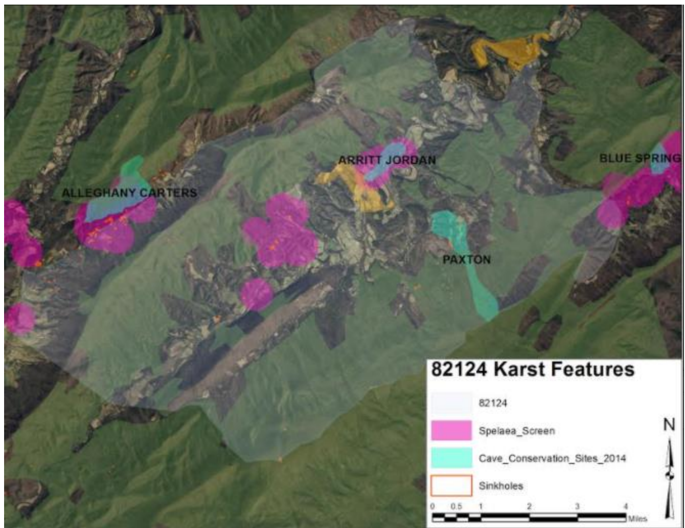
Figure 1: Karst Features
