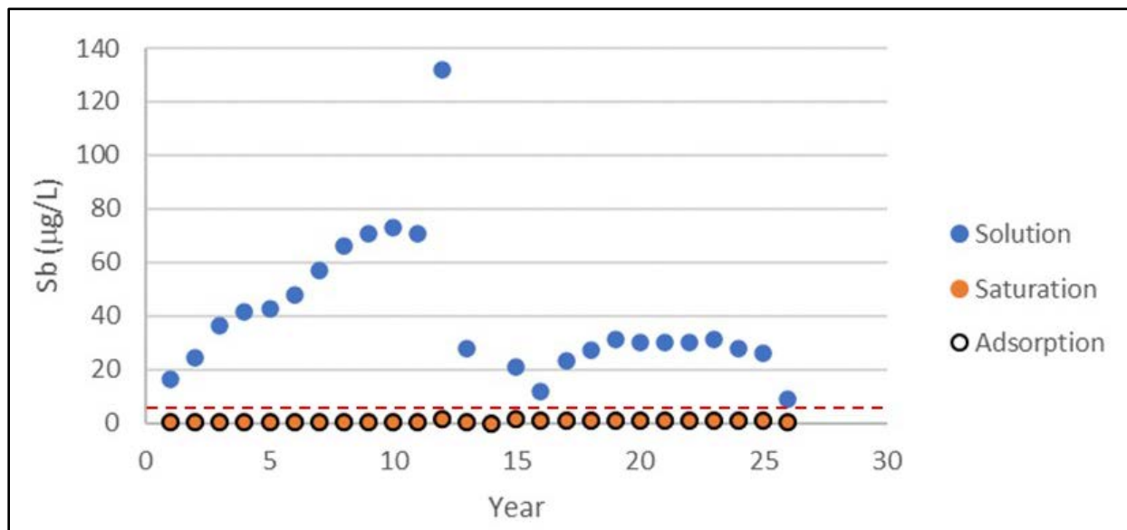
Figure 1. Predicted antimony concentrations in groundwater under the Hangar Flats DRSF over time. The dashed red line is the groundwater quality standard of 6 µg/L (DEIS, Table 3.9-2, p. 3.9-15).
