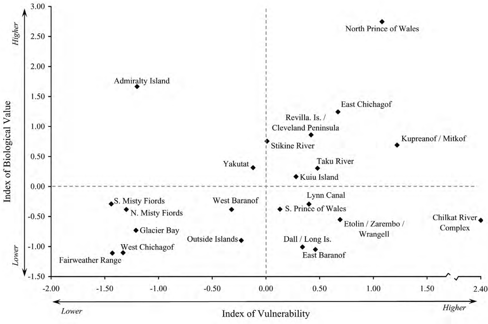
FIGURE 3-2 The index of biological value is a combined index based on relative contribution of each province to the regional distribution of habitat values, and the index of vulnerability reflects the percent of habitat values within each province that are designated within development Land Use Designations (LUDs) or private lands. Values were normalized to facilitate comparison among provinces.
