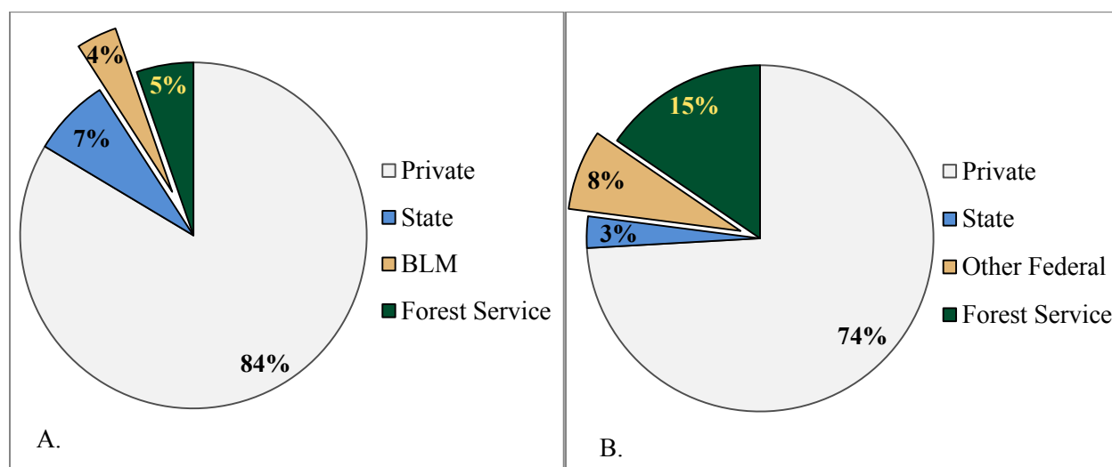
Figure 3-17. Proportion of estimated greenhouse gas emissions from (a) timber harvest and (b) prescribed burning by different entities
