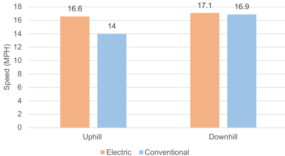
Figure 12. Average uphill and downhill speeds for electric and conventional bikes on the US 36 Bikeway [n(electric uphill)=8, n(conventional uphill)=36, n(electric downhill)= 13, n(conventional downhill)=50].
