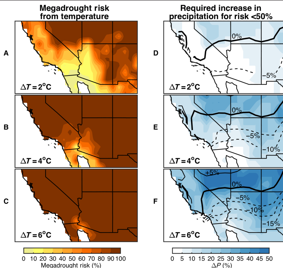
Fig. 4. Maps of megadrought risk for the American Southwest under different levels of warming, and the required increase in precipitation for that warming. (A to C) Maps of megadrought risk for the entire American Southwest domain at constant (historical) precipitation climatology ( \Delta P = 0\% ) and various levels of warming. These estimates are based on the Monte Carlo procedure of observational and reanalysis data, not on CMIP5 (see Materials and Methods). (D to F) Increases in precipitation (blue shading) needed to maintain megadrought risks below 50% for different levels of regional warming. Contours map the projected changes in precipitation derived from the multimodel CMIP5 mean and are shown for reference at each level of temperature change.
