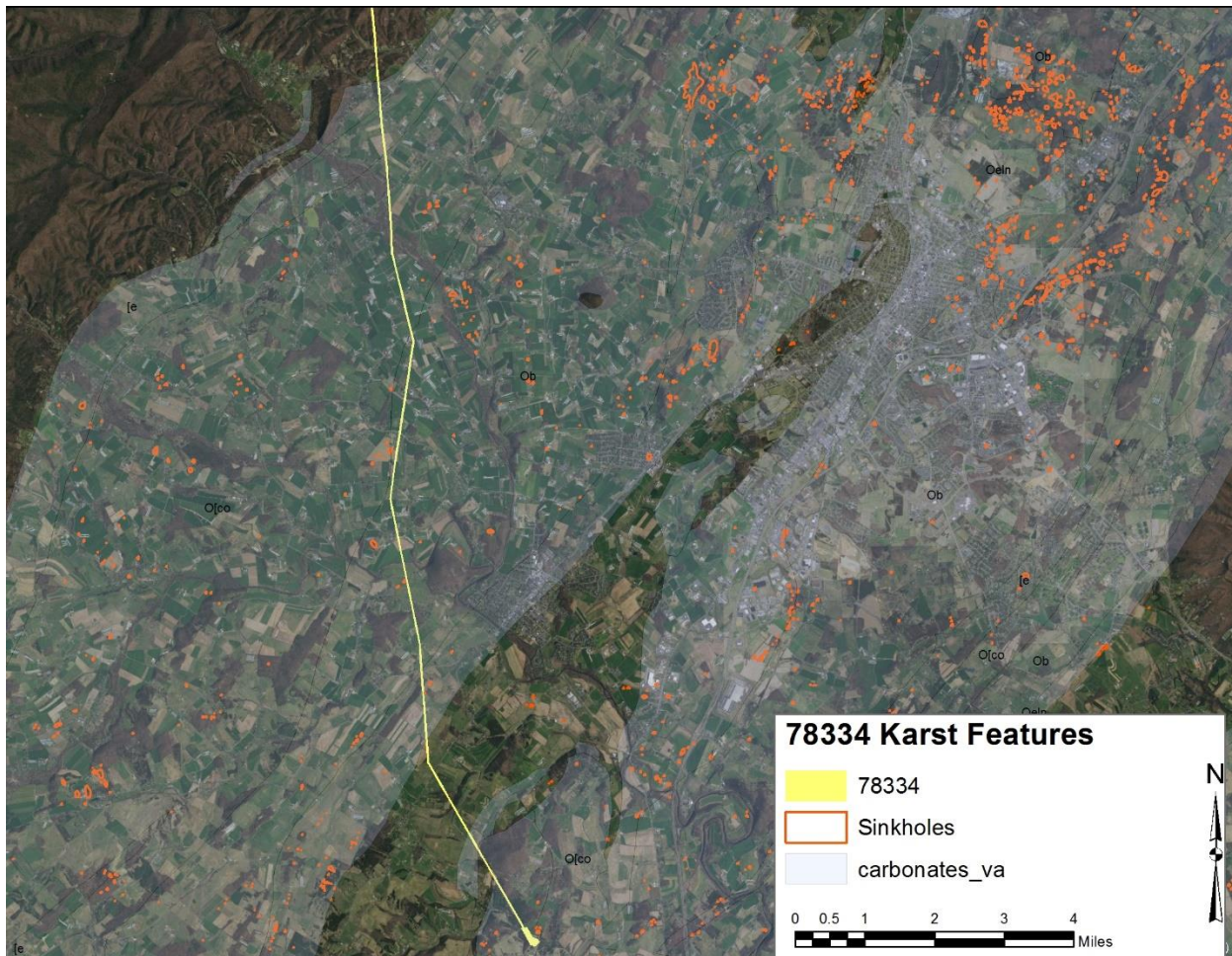
Figure 1. Carbonate rock coverage and the southern portion of the project site.
