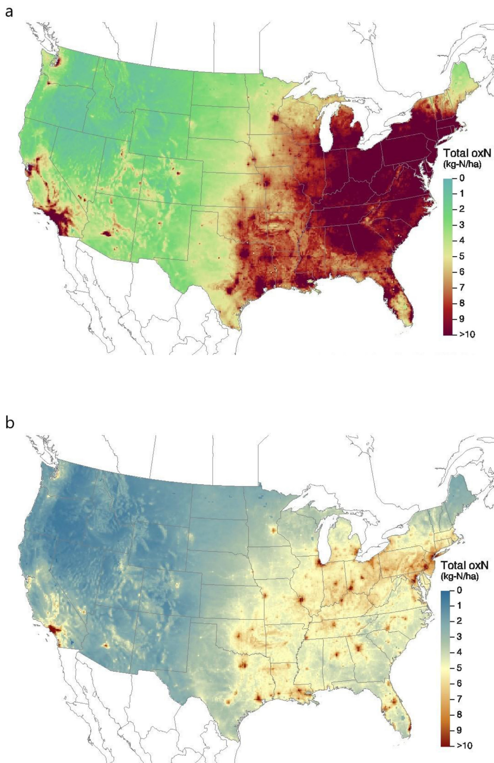
Fig. 2. Total deposition of \text{NO}_x for 2000 (a) and 2014 (b). Maps were taken from the National Atmospheric Deposition Program ( http://nadp.slh.wisc.edu/ ).
