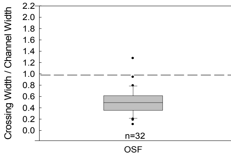
Figure C4. Crossing width to bankfull channel width ratio for crossings surveyed in summer 2007 on the Ozark-St. Francis National Forest (excluding fords, vented fords, and multiple structure crossings). A ratio of 1.0 (dashed line) or greater indicates the crossing structure opening is greater than or equal to the bankfull channel width. The top and bottom of the boxes represent the 25th and 75th percentiles, the bar in the center of each box represents the median, whiskers represent the 10th and 90th percentiles, and closed circles represent the entire range of the data.
