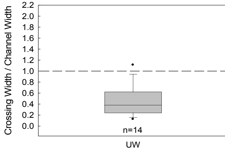
Figure D4. Crossing width to bankfull channel width ratio for crossings surveyed in summer 2007 on the Uwharrie National Forest (excluding fords, vented fords, and multiple structure crossings). A ratio of 1.0 (dashed line) or greater indicates the crossing structure opening is greater than or equal to the bankfull channel width. The top and bottom of the boxes represent the 25th and 75th percentiles, the bar in the center of each box represents the median, whiskers represent the 10th and 90th percentiles, and closed circles represent the entire range of the data.
