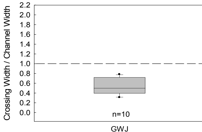
Figure G4. Crossing width to bankfull channel width ratio for crossings surveyed in summer 2007 on the George Washington-Jefferson National Forest in Virginia (excluding fords, vented fords, and multiple structure crossings). A ratio of 1.0 (dashed line) or greater indicates the crossing structure opening is greater than or equal to the bankfull channel width. The top and bottom of the boxes represent the 25th and 75th percentiles, the bar in the center of each box represents the median, whiskers represent the 10th and 90th percentiles, and closed circles represent the entire range of the data.
