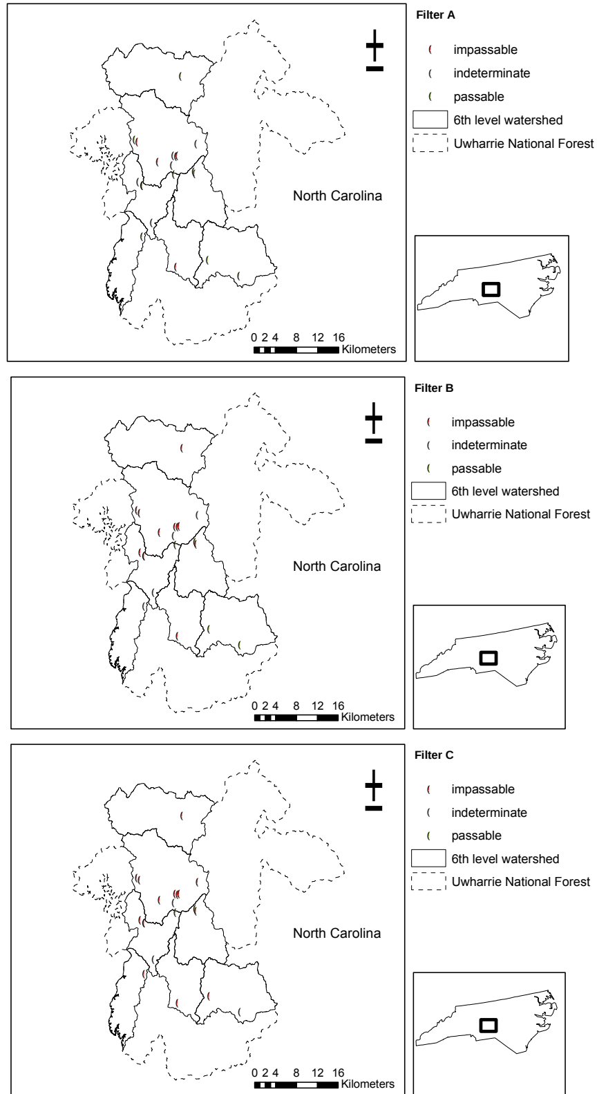
Figure D6. Location of crossings classified for fish passage by coarse filters A, B, and C within 6th level watersheds on the Uwharrie National Forest, summer 2007.
