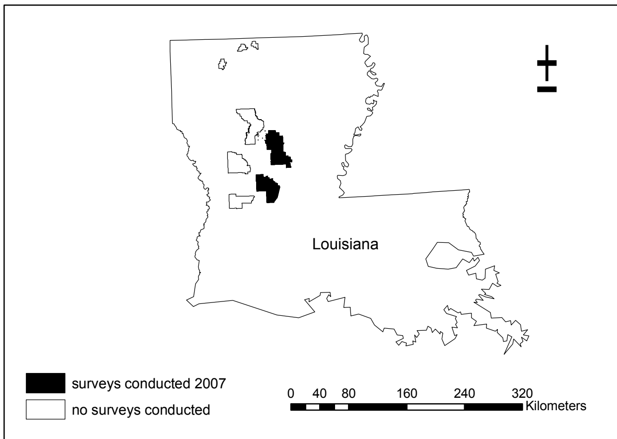
Figure F1. Ranger Districts on the Kisatchie National Forest, Louisiana where road-stream crossing surveys were conducted, summer 2007.
