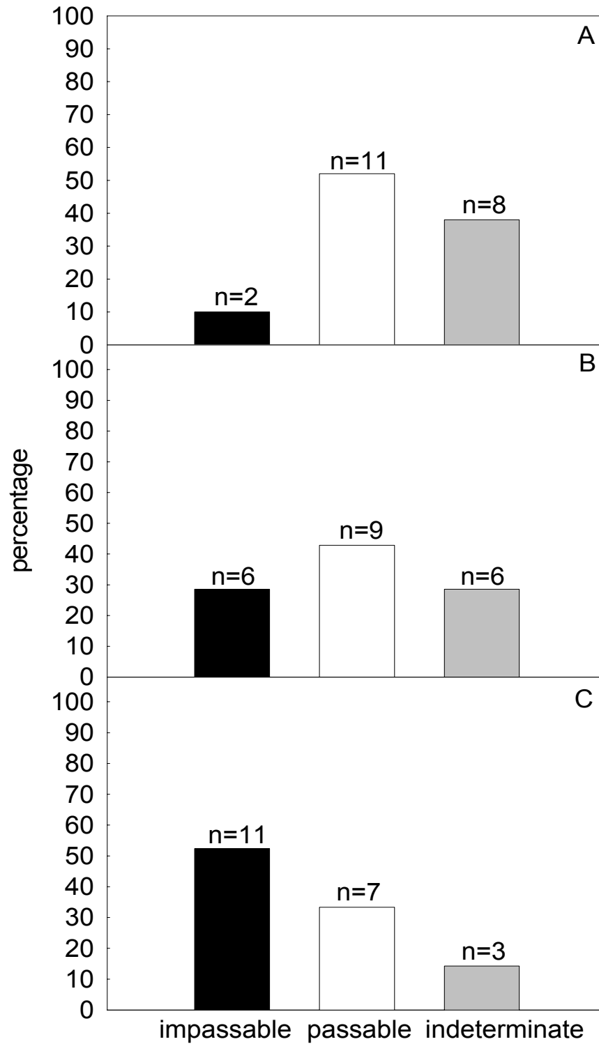
Figure E2. Percentage of crossings classified as impassable, passable, or indeterminate for Filter A, B, and C; Sam Houston National Forest, Texas, summer 2007 (N= 21).
