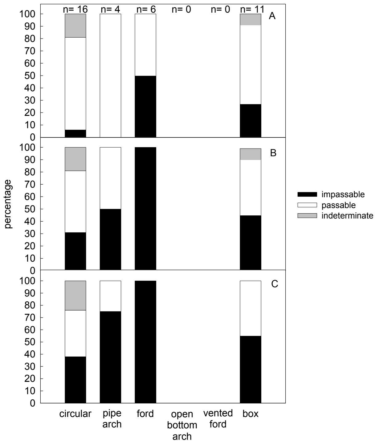
Figure A3. Percentage of each crossing type classified as impassable, passable, or indeterminate for Filter A, B, and C; Land Between the Lakes National Recreation Area, Kentucky, summer 2007 (N= 37).
