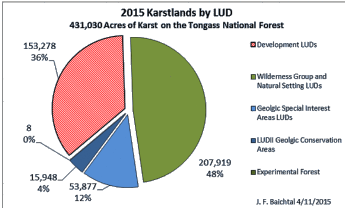
Karst and Cave Figure 1. 2015 karst lands by land use designation (LUD)
