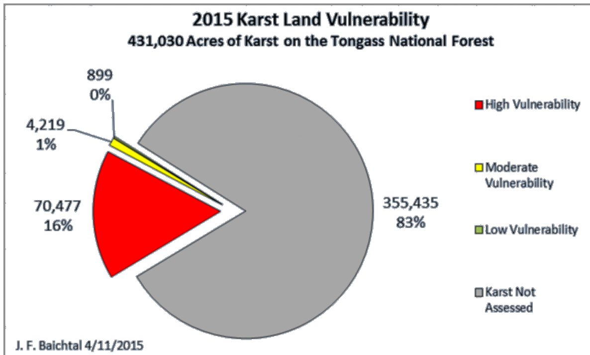
Karst and Cave Figure 2. 2015 karst land vulnerability
