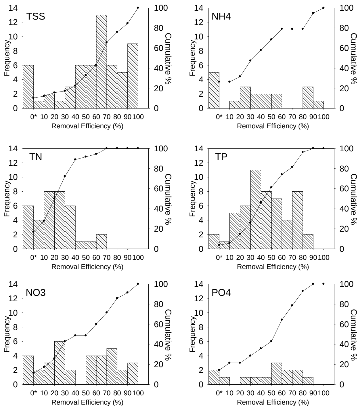
Fig. 2. Frequency analysis of removal efficiencies for single-site studies. Frequency (number of reported values) in removal-efficiency increments of 10 % (e.g. 10-20%, 20-30%, etc.) is plotted on the left axis and as bars. The cumulative percentage of studies reporting values within each removal-efficiency increment is plotted on the right axis as circular symbols connected by lines. The 0* category includes any studies reporting efficiencies of 0% or less (i.e. net efflux).
