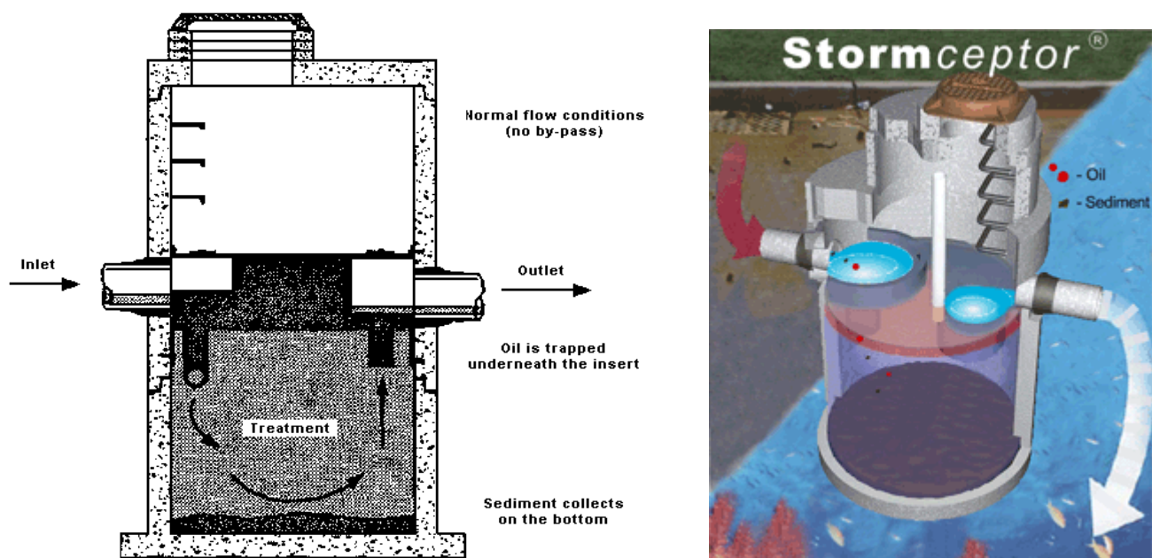
Stormceptor® hydrodynamic device. The unit is installed below grade surface and accessed via a manhole; note ladder in upper chamber for scale. Source: http://www.fhwa.dot.gov/environment/ultraurb/3fs14.htm and http://www.rinkerstormceptor.com/images/flow_1.gif .
