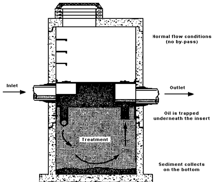
Stormceptor® hydrodynamic device. The unit is installed below grade surface and accessed via a manhole; note ladder in upper chamber for scale. Source:
