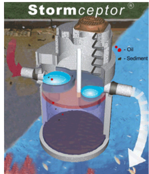
Stormceptor® hydrodynamic device. The unit is installed below grade surface and accessed via a manhole; note ladder in upper chamber for scale. Source:
