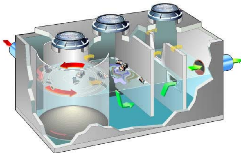
Vortechs® hydrodynamic device. This is a multi-chambered device installed below-ground that is accessed via manholes. Source: http://www.epa.gov/NE/assistance/ceitts/images/techsimgs/vortechs2.jpg .
