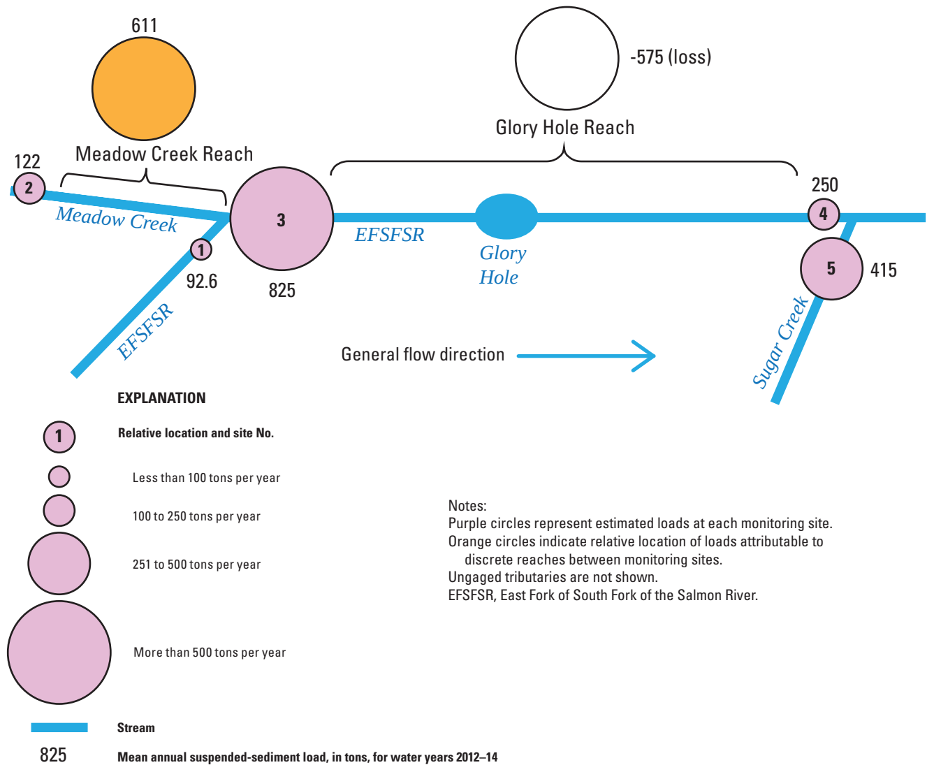
Figure 13. Estimated mean annual suspended sediment loads at monitoring sites in the Stibnite mining area, central Idaho, 2012–14. Site names and locations are shown in table 1 and figure 1 , respectively.
