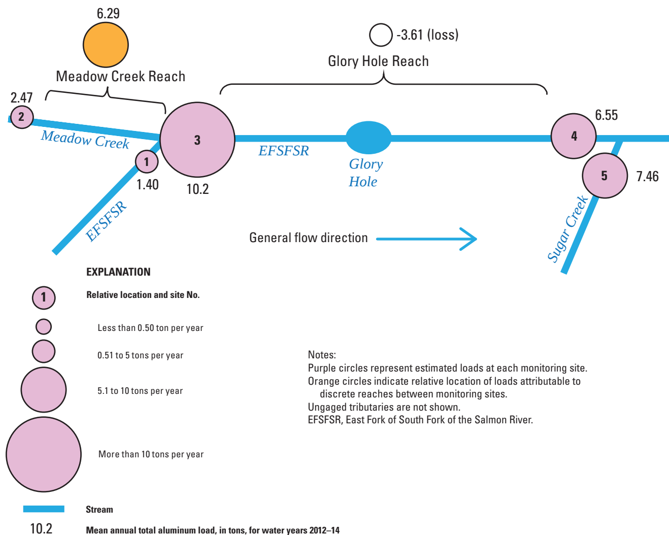
Figure 14. Estimated mean annual total aluminum loads at monitoring sites in the Stibnite mining area, central Idaho, 2012–14. Site names and locations are shown in table 1 and figure 1 , respectively.
