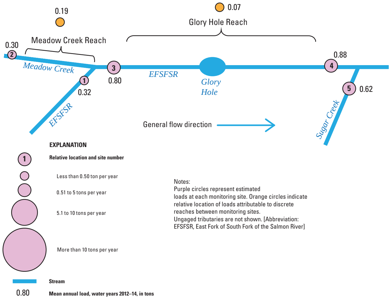
Figure 15. Estimated mean annual dissolved aluminum loads at monitoring sites in the Stibnite mining area, central Idaho, 2012–14. Site names and locations are shown in table 1 and figure 1 , respectively.
