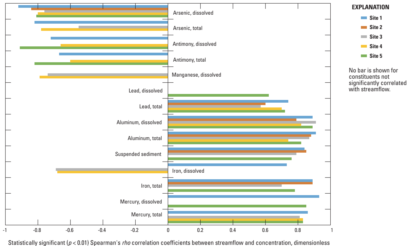
Figure 6. Correlation between streamflow and constituent concentrations for trace elements and suspended sediment in streams in the Stibnite mining area, central Idaho, 2012–14. Site names and locations are shown in table 1 and figure 1 , respectively.
